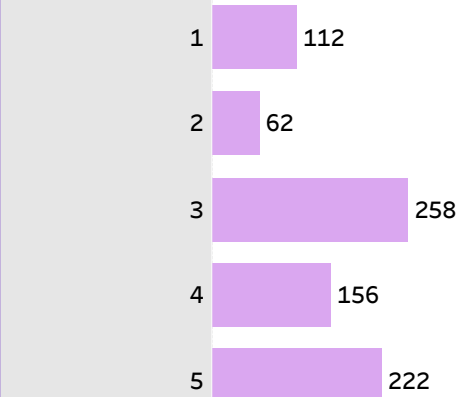
Satisfaction Score
